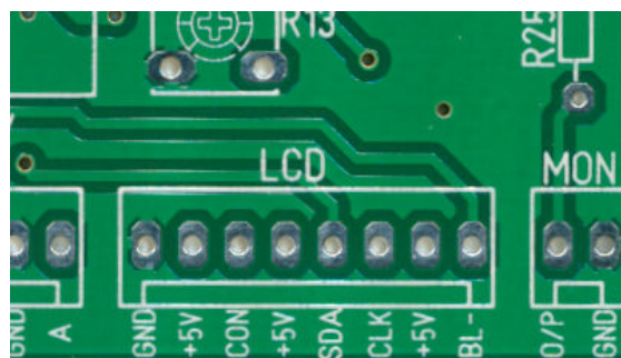
TIM 2015 component side
