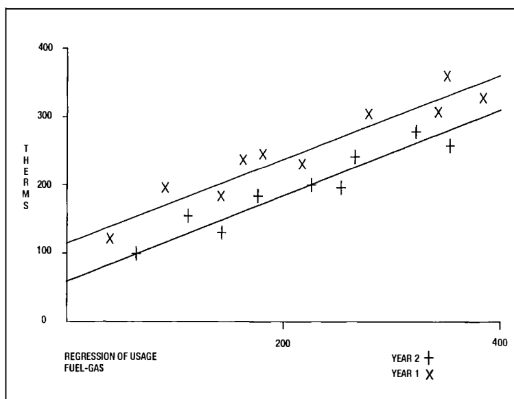
Figure 7—Regression analysis
