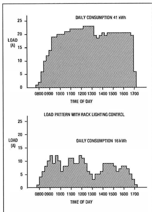
Figure 7—Rack lighting control
