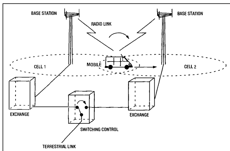
Figure 4 A schematic diagram showing the handover process
