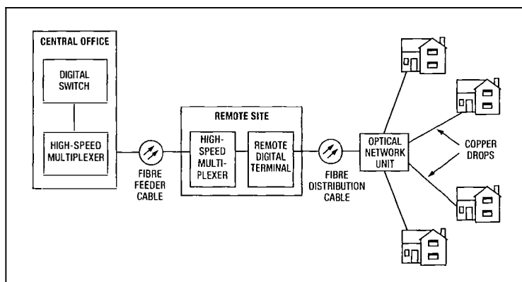
Figure 5 Fibre to the curb
