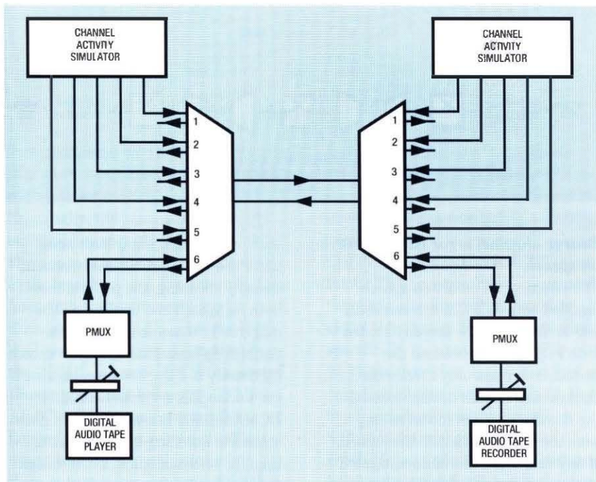
Figure 2—Typical test setup
