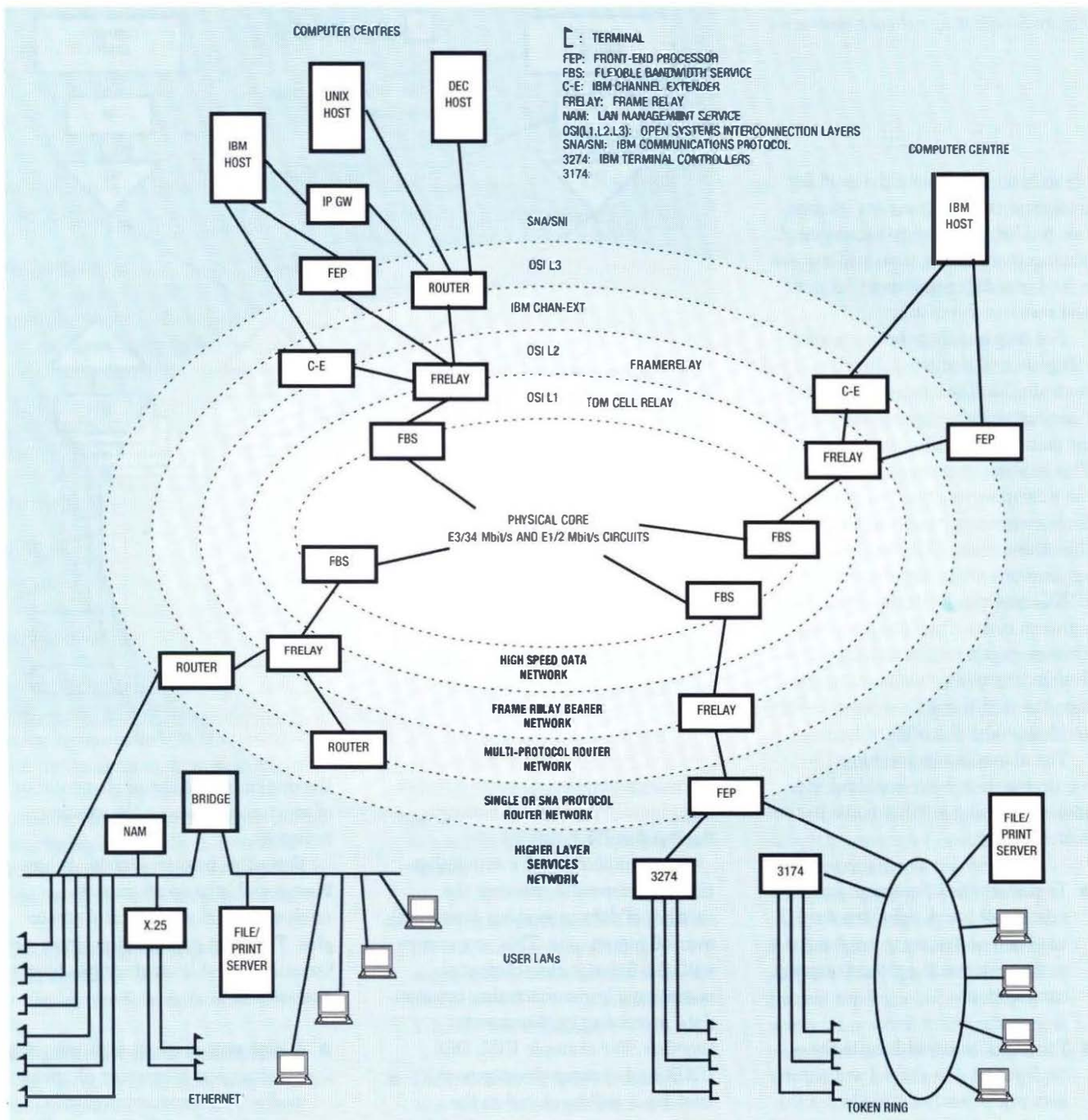
Figure 6—BT corporate data network
