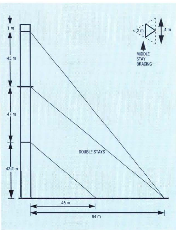
Figure 4—Onshore mast design parameters
