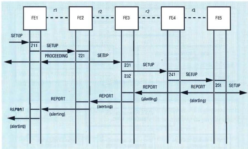
Figure 4—Information flow for basic call
