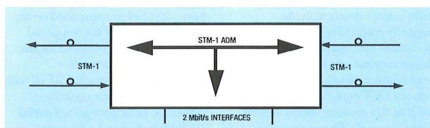
Figure 11—NISTAR add/drop multiplex
