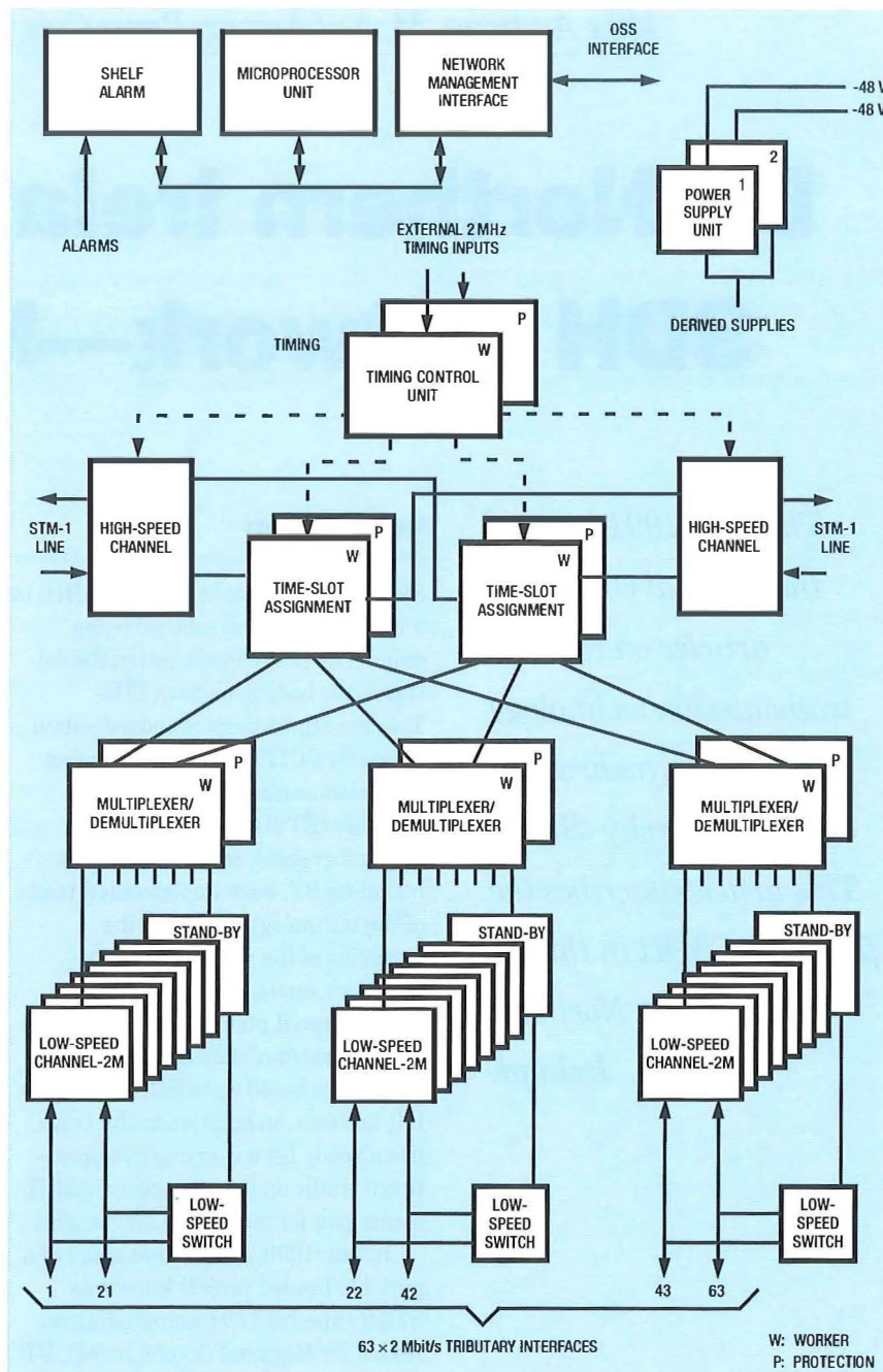
Figure 2—Block diagram of NISTAR add/drop multiplexer
