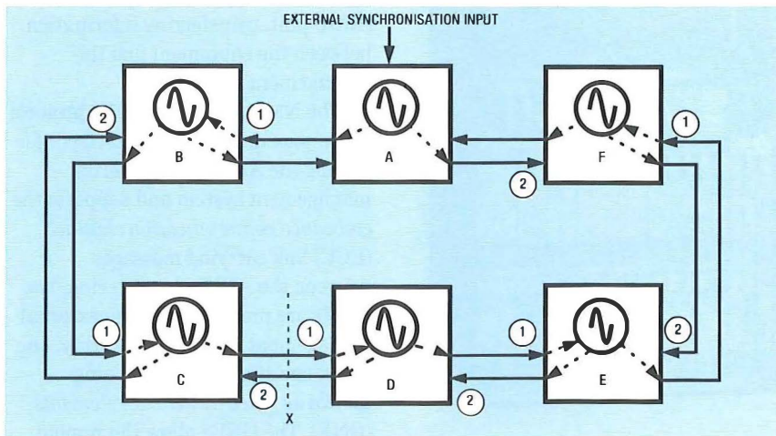
Figure 6—Synchronisation failure
