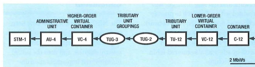
Figure 10—NISTAR equipment multiplexing hierarchy
