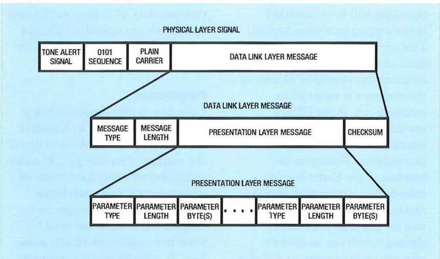
Figure 4—Caller Display signal format
