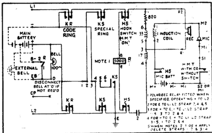
SCHEMATIC
